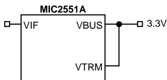
Figure 8. Powering MIC2551A from External 3.3V
