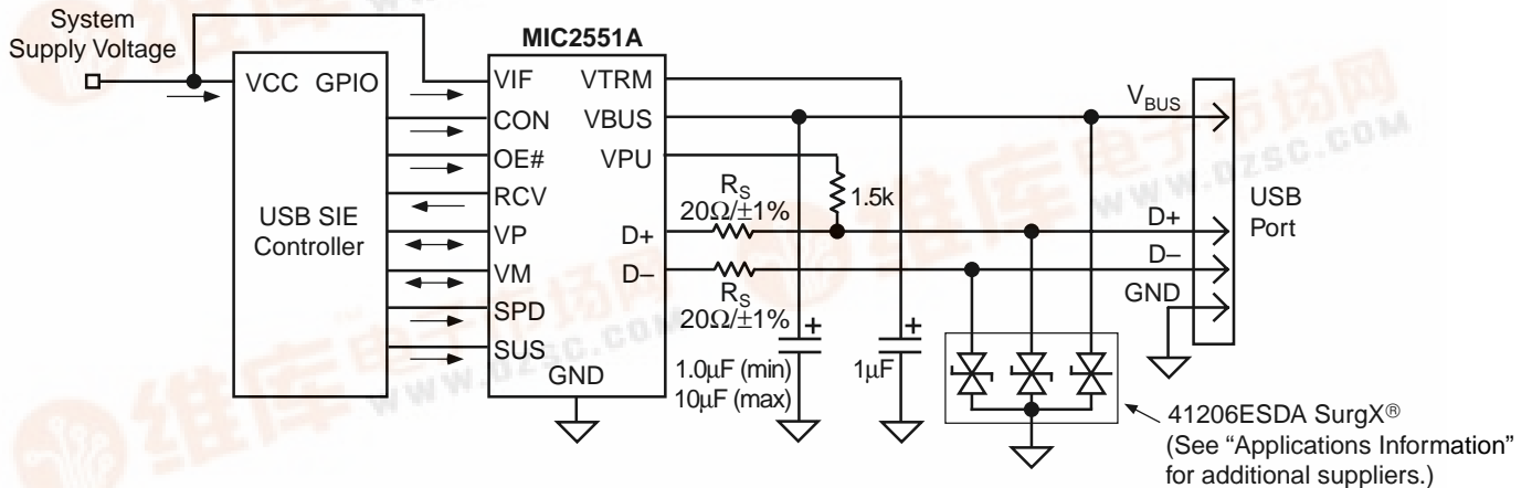
Typical Application Circuit
