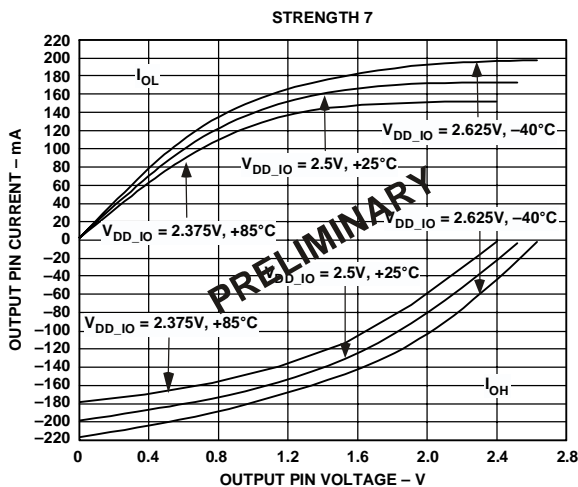
Figure 29. Typical Drive Currents at Strength 7
