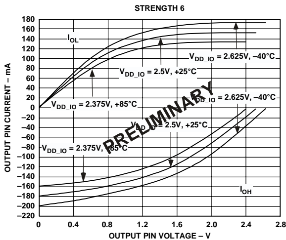
Figure 28. Typical Drive Currents at Strength 6
