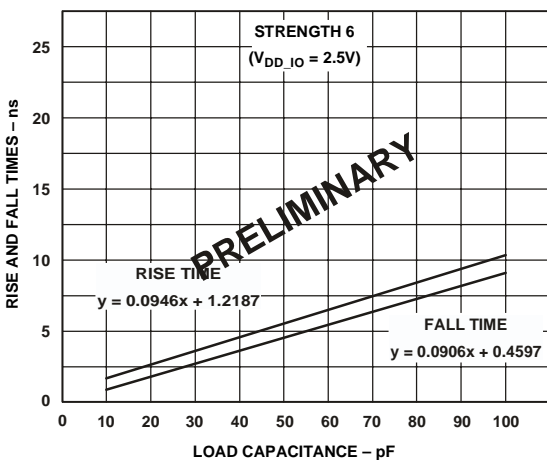
Figure 39. Typical Output Rise and Fall Time (10%–90%, V_{DD\_IO} = 2.5\text{ V} ) vs. Load Capacitance at Strength 6
