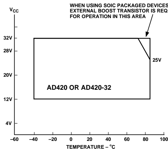
Figure 13. Safe Operating Region
