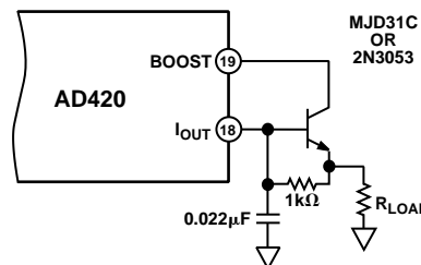
Figure 12. External Boost Configuration
