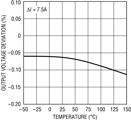
LT1083 Load Regulation
