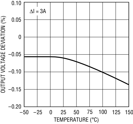
LT1085 Load Regulation
