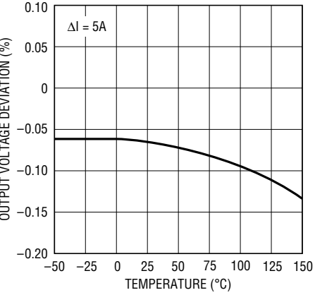
LT1084 Load Regulation
