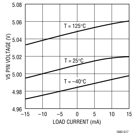
V5 Voltage vs Load Current
