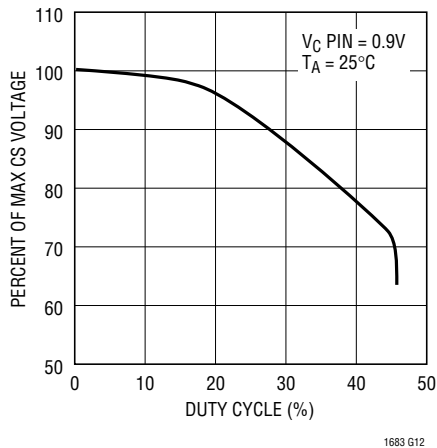
Slope Compensation
