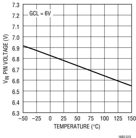
Gate Drive Undervoltage Lockout Voltage vs Temperature
