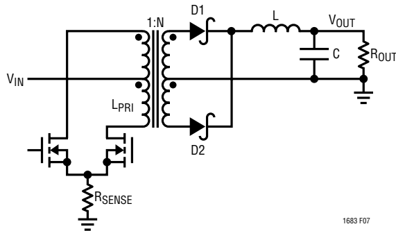
Figure 7. Push-Pull Topology
