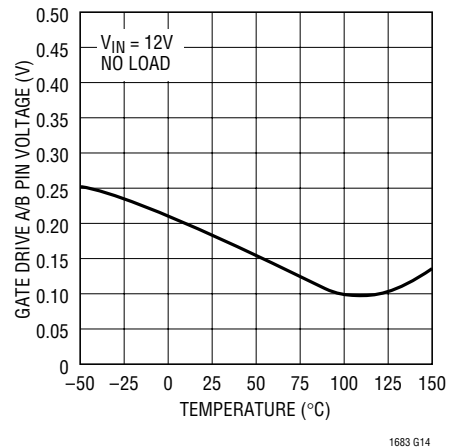
Gate Drive A/B Low Voltage vs Temperature
