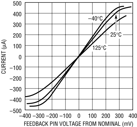
Error Amp Output Current vs Feedback Pin Voltage from Nominal
