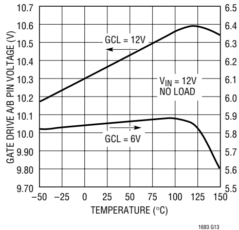
Gate Drive A/B High Voltage vs Temperature
