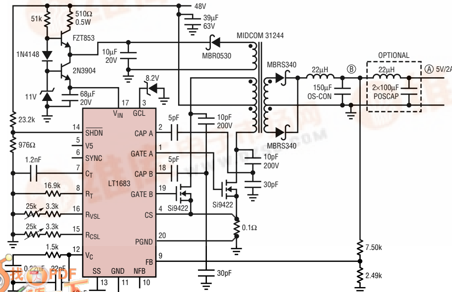
Ultralow Noise 48V to 5V DC/DC Converter
