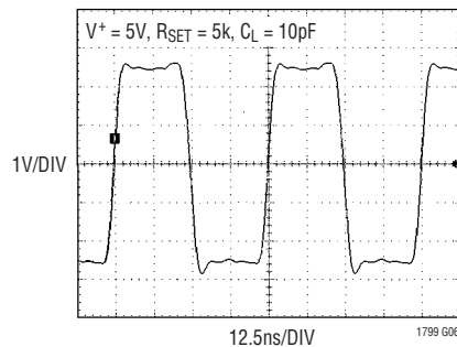
LTC1799 Output Operating at 20MHz, V S = 5V
