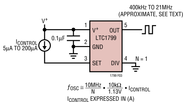
Figure 3. Current Controlled Oscillator
