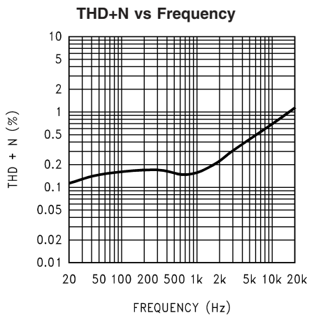
200470D4 V_{DD} = 12V, R_L = 8\Omega, BTL operation, BTLA_V = 20, P_{OUT} = 3W
