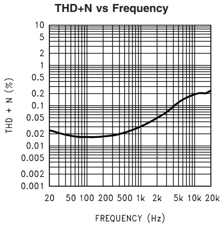
200470B2 V_{DD} = 12V, R_L = 8\Omega, BTL operation, P_{OUT} = 1W
