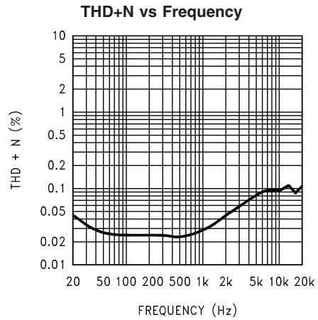
200470B3 V_{DD} = 12V, R_L = 8\Omega, BTL operation, P_{OUT} = 3W
