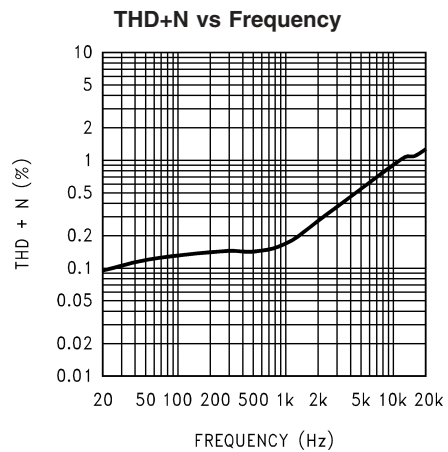
200470D5 V_{DD} = 12V, R_L = 8\Omega, BTL operation, BTLA_V = 20, P_{OUT} = 1W
