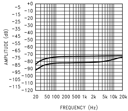
200470A2 V_{DD} = 16V, R_L = 8\Omega, P_{OUT} = 1W, SE operation at (from top to bottom at 1kHz): V_{INB} driven, V_{OUTA} measured; V_{INA} driven, V_{OUTB} measured
