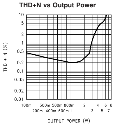
200470D3 V_{DD} = 16V, R_L = 8\Omega, BTL operation, f_{IN} = 1kHz, BTLA_V = 20
