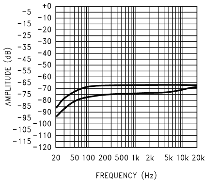
20047097 V_{DD} = 16V, R_L = 4\Omega, P_{OUT} = 1W, SE operation at (from top to bottom at 1kHz): V_{INB} driven, V_{OUTA} measured; V_{INA} driven, V_{OUTB} measured
