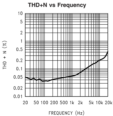
200470B4 V_{DD} = 12V, R_L = 8\Omega, BTL operation, P_{OUT} = 5W
