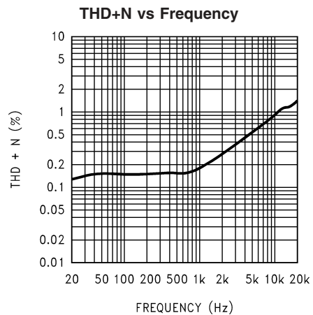
200470D6 V_{DD} = 12V, R_L = 8\Omega, BTL operation, BTLA_V = 20, P_{OUT} = 5W
