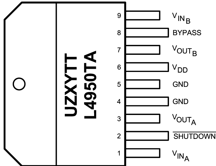
Plastic Package, TO-220
