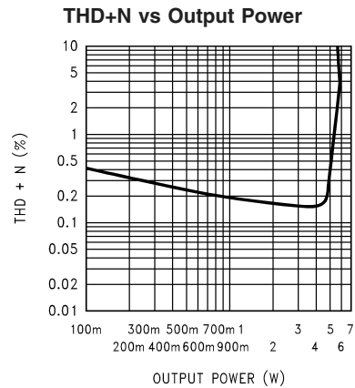
200470C9 V_{DD} = 16V, R_L = 4\Omega, A_V = 10 SE operation, f_{IN} = 1kHz, both channels driven and loaded (average shown)
