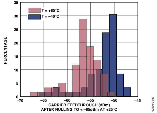
Figure 40. Carrier Feedthrough Distribution at Temperature Extremes, After Carrier Feedthrough Nulled to <-65\text{ dBm} at T_A = 25^\circ\text{C} . ( F_{LO} = 2140\text{ MHz} , I and Q Inputs at a bias of 400\text{ mV} )
