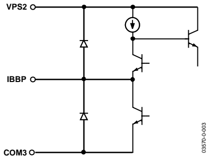
Figure 3. Circuit A
