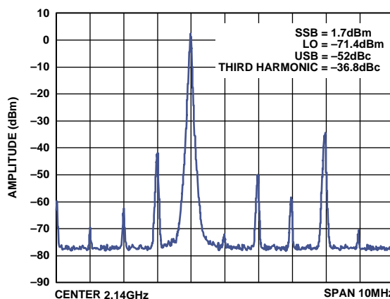
Figure 55. AD8349 Single Sideband Spectrum at 2140 MHz after LO Nulling
