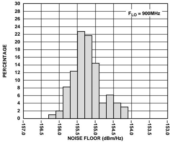
Figure 25. 20 MHz Offset Noise Floor Distribution at F_{LO} = 900\text{ MHz} (I and Q Inputs at a Bias of 400 mV, T_A = 25^\circ\text{C} )
