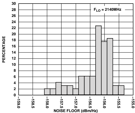
Figure 27. 20 MHz Offset Noise Floor Distribution at F_{LO} = 2140\text{ MHz} (I and Q Inputs at a Bias of 400 mV, T_A = 25^\circ\text{C} )
