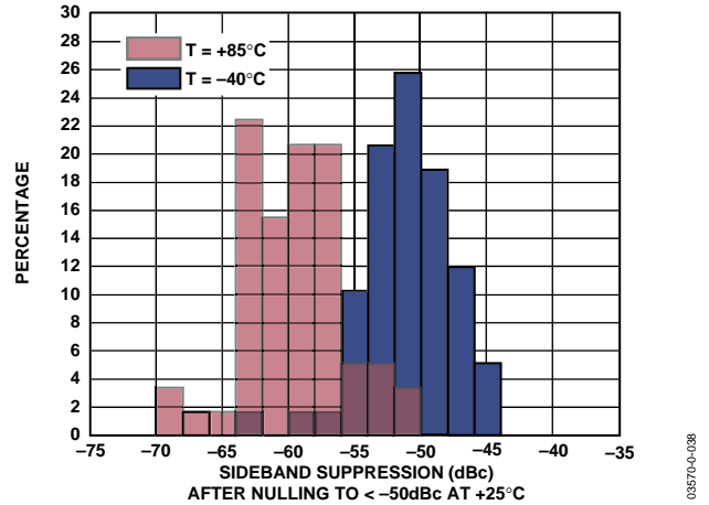
Figure 41. Sideband Suppression Distribution at Temperature Extremes, After Sideband Suppression Nulled to <-50\text{ dBc} at T_A = 25^\circ\text{C} . ( F_{LO} = 2140\text{ MHz} , F_{BB} = 1\text{ MHz} , I and Q Inputs biased at 0.4\text{ V} )
