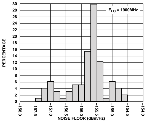
Figure 26. 20 MHz Offset Noise Floor Distribution at F_{LO} = 1900\text{ MHz} (I and Q Inputs at a Bias of 400 mV, T_A = 25^\circ\text{C} )
