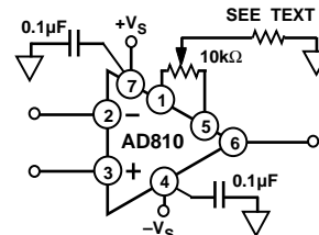
Offset Null Configuration
