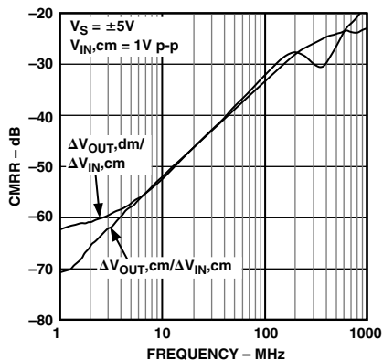
Figure 27. CMRR vs. Frequency
