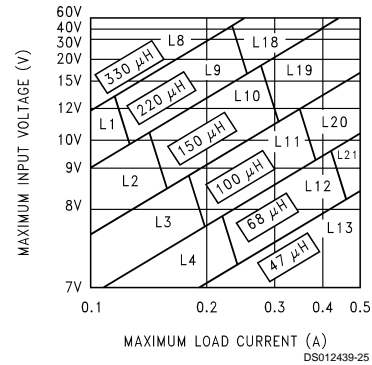
FIGURE 5. LM2594/LM2594HV-5.0
