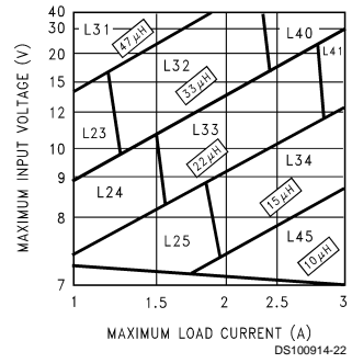
FIGURE 4. LM2676-5.0
