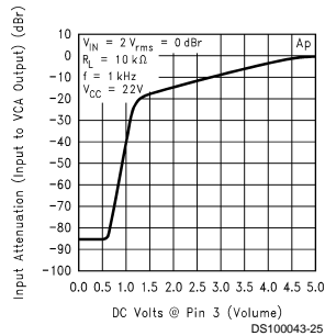
Volume Attenuation vs DC Voltage
