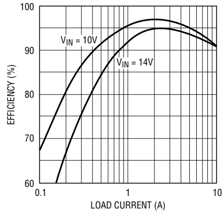
Figure 19. All N-Channel 5V/8A Efficiency
