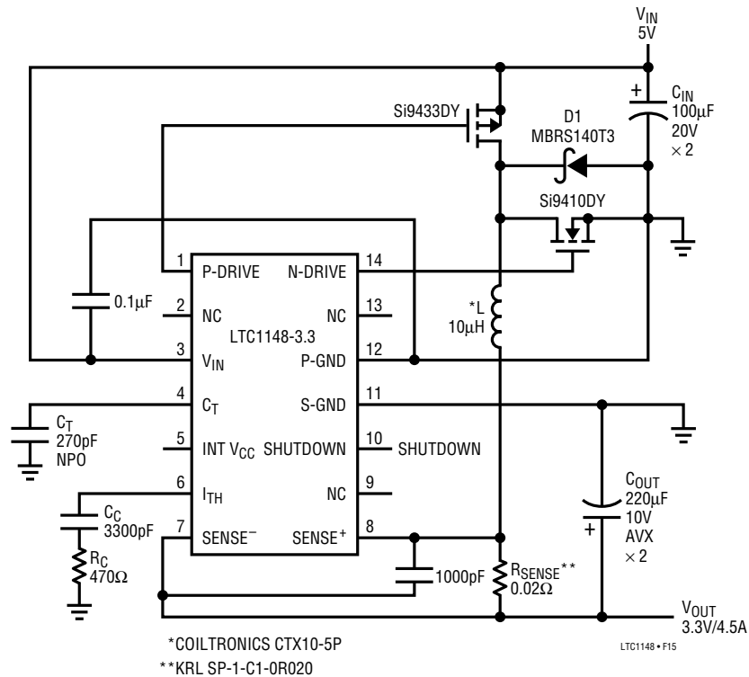
Figure 15. High Efficiency 5V to 3.3V/4.5A Converter
