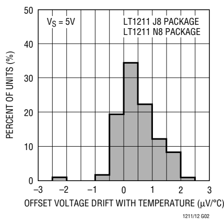
Distribution of Offset Voltage Drift with Temperature
