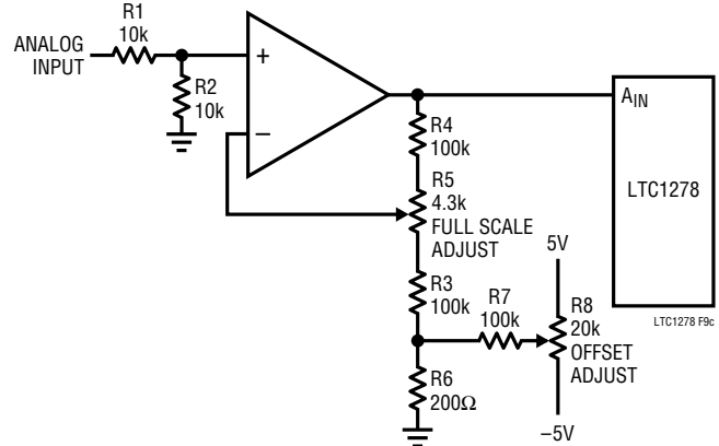
Figure 9c. LTC1278 Bipolar Offset and Full Scale Adjust Circuit
