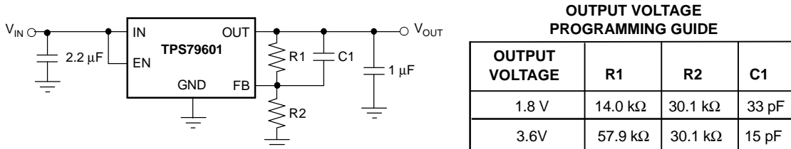
Figure 23. TPS79601 Adjustable LDO Regulator Programming
