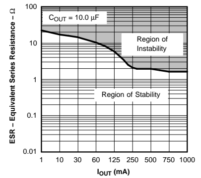
TPS79630 TYPICAL REGIONS OF STABILITY EQUIVALENT SERIES RESISTANCE (ESR) VS OUTPUT CURRENT
