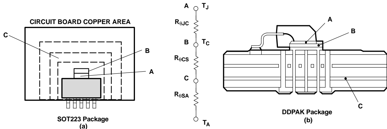
Figure 24. Thermal Resistances
