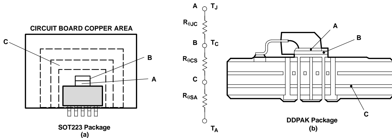
Figure 19. Thermal Resistances
