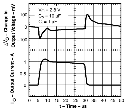
TPS72618 LOAD TRANSIENT RESPONSE
