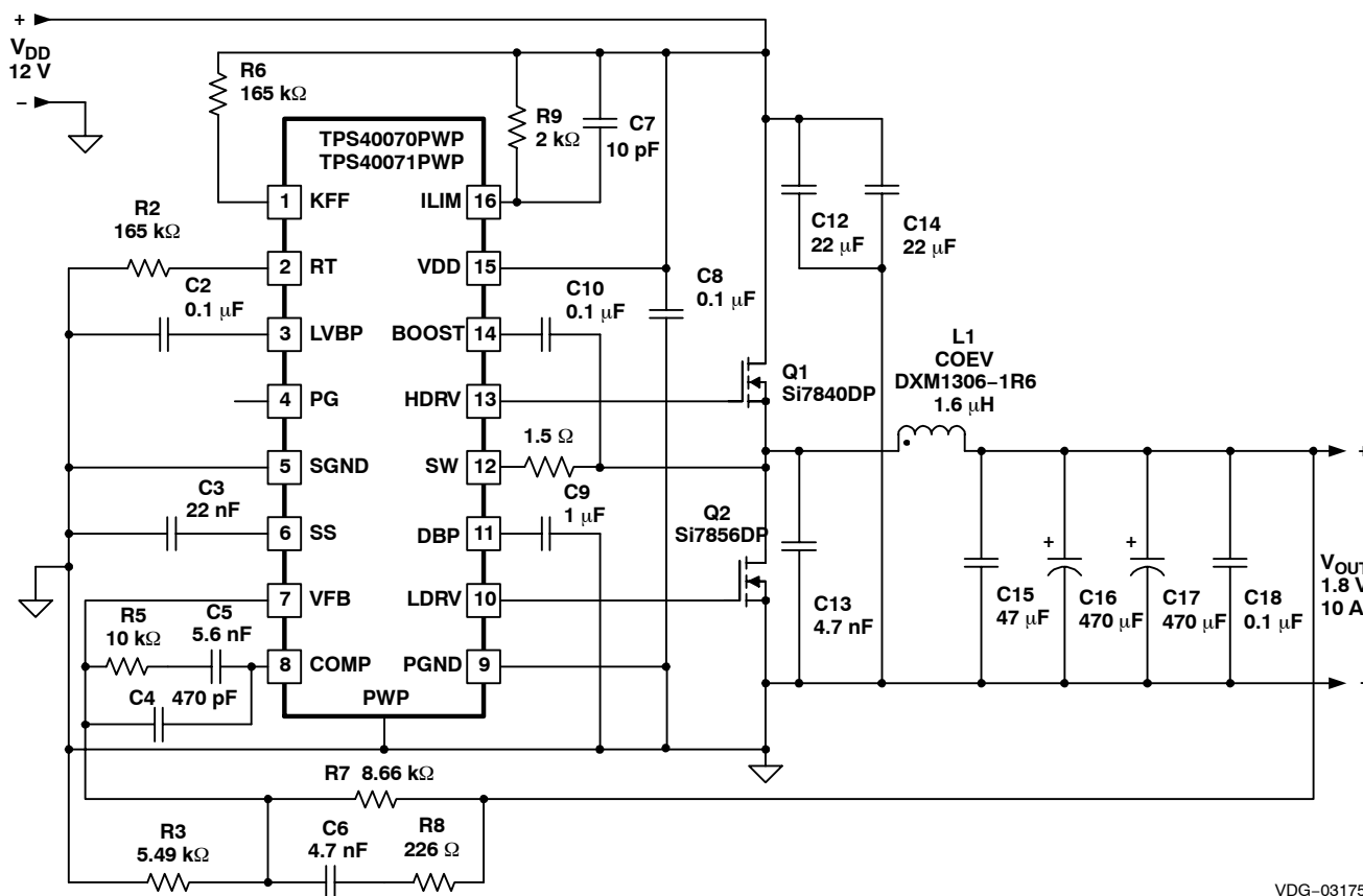
Figure 14. 300 kHz, 12 V to 1.8 V
