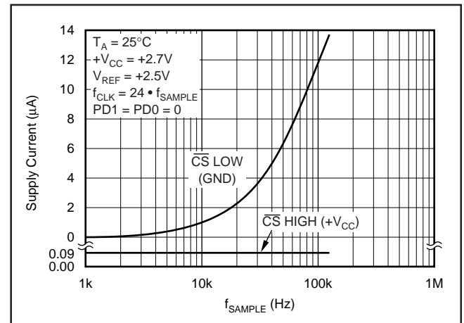
FIGURE 11. Supply Current vs State of \overline{\text{CS}} .
