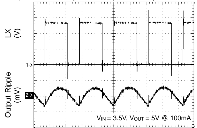
LX & Output Ripple
