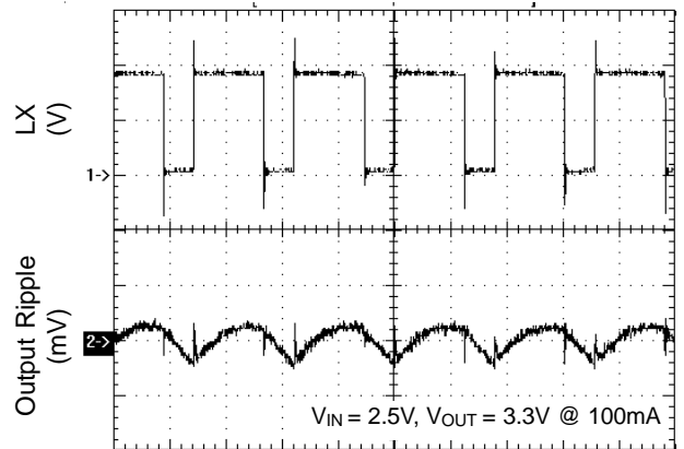
LX & Output Ripple
