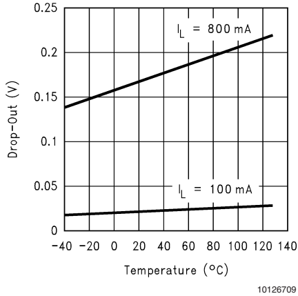
Drop-Out Voltage Vs Temperature for Different Load Currents
