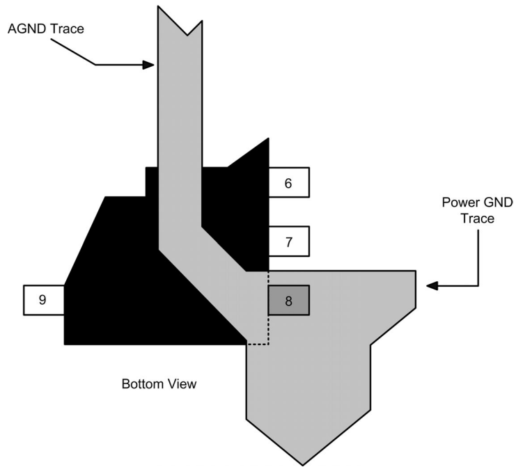
FIGURE 4. Single Layer Layout
