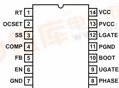
ISL8104 (14 LD NARROW SOIC AND 16 LD QFN) TOP VIEW
