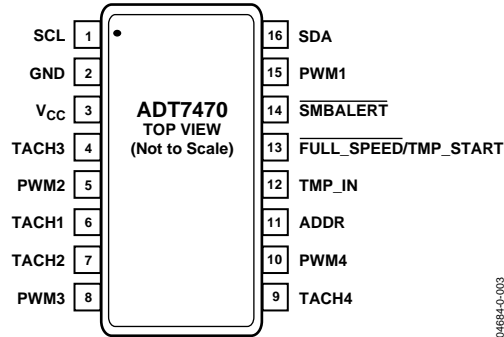
Figure 3. Pin Configuration
