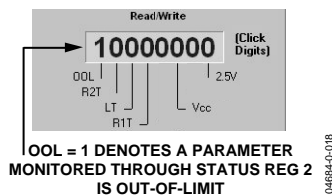
Figure 19. Interrupt Status Register 1
