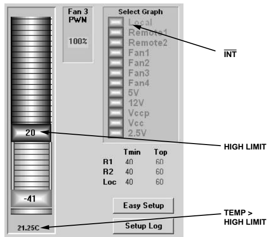
Figure 18. Temperature > High Limit— \overline{INT} Occurs
