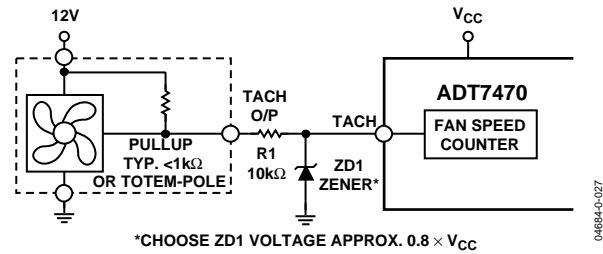
Figure 28. Fan with Strong Tach. Pull-up to > V_{CC} or Totem-Pole Output, Clamped with Zener and Resistor.
