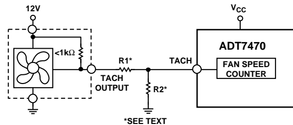
Figure 29. Fan with Strong Tach. Pull-up to > V_{CC} or Totem-Pole Output, Attenuated with R1/R2 .
