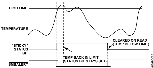
Figure 21. SMBALERT and Status Bit Behavior
