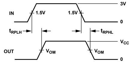
Figure 16. Receiver Propagation Delay
