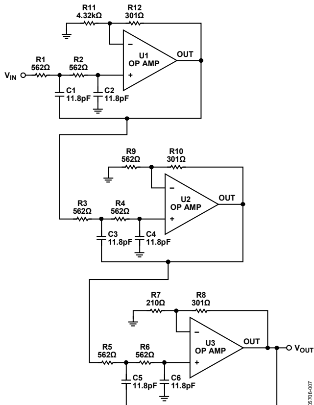
Figure 48. 20 MHz, 6-Pole Low-Pass Filter
