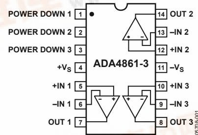
Figure 1. SOIC (R-14)
