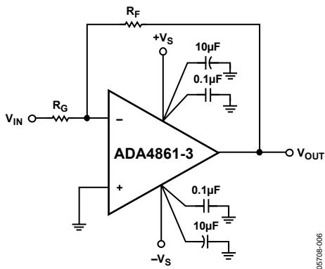
Figure 47. Inverting Gain
