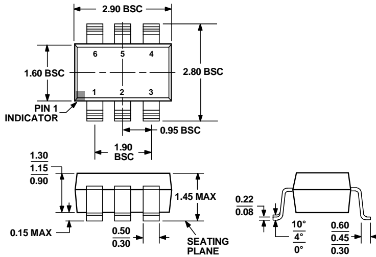
Figure 46. 6-Lead Small Outline Transistor Package [SOT-23] (RJ-6) Dimensions shown in millimeters
