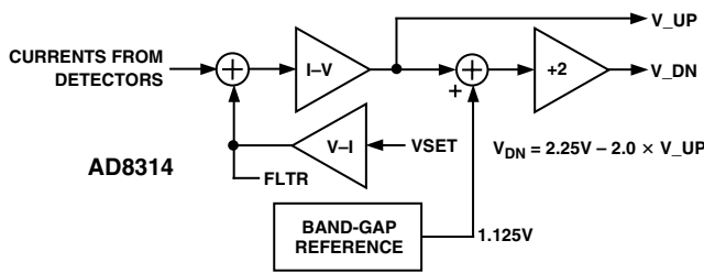
Figure 2. Output Interfaces
