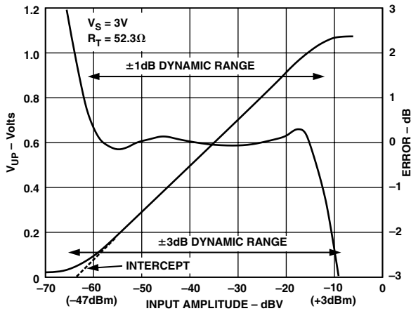
Figure 5. V_{UP} and Log Conformance Error vs. Input Level vs. Input Level at 900 MHz
