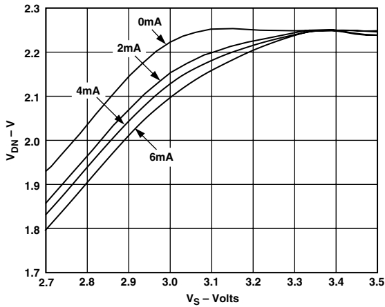
TPC 19. Maximum V_{DN} Voltage vs. V_S by Load Current
