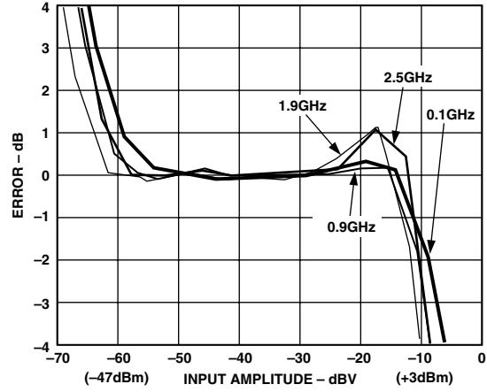
TPC 4. Log Conformance vs. Input Amplitude
