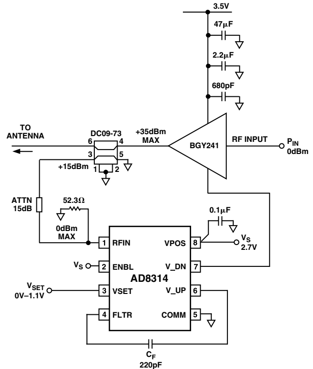
Figure 12. A Single Mode Power Amplifier Control Circuit
