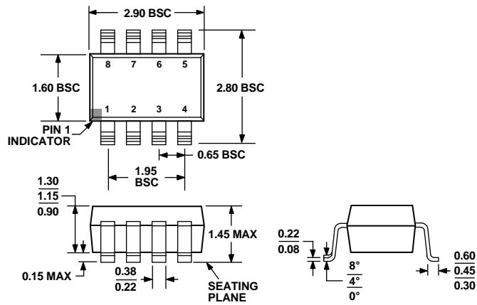
Figure 36. 8-Lead Small Outline Transistor Package [SOT-23] (RT-8)
