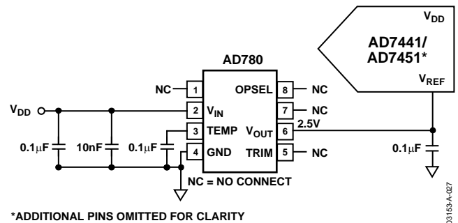
Figure 27. Typical V_{\text{REF}} Connection Diagram for V_{\text{DD}} = 5 V
