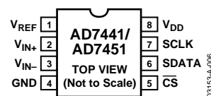
Figure 6. 8-Lead MSOP
