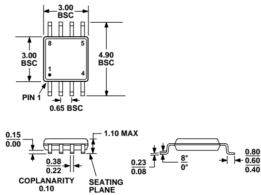
Figure 37. 8-Lead Mini Small Outline Package [MSOP] (RM-8)
