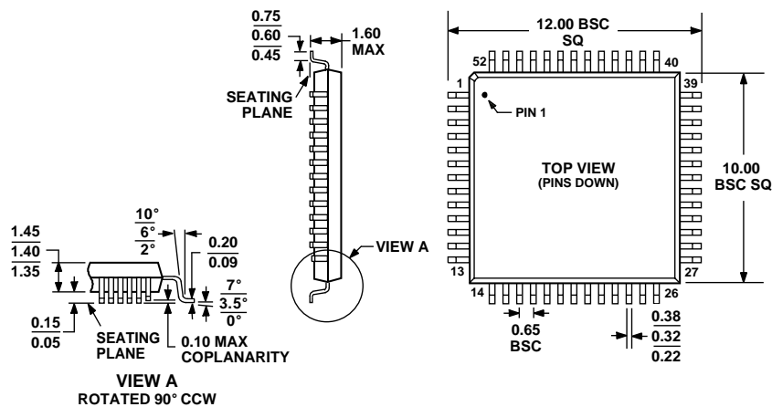
Figure 14. 52 Lead LQFP Package Dimensions shown in millimeters
