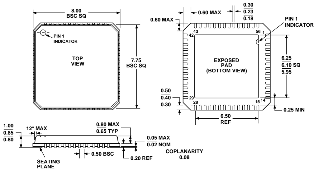
Figure 13. 56 Lead LFCSP Package Dimensions shown in millimeters
