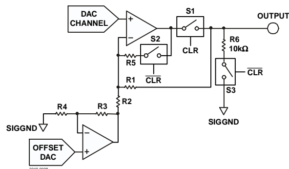
Figure 9. Output Amplifier and Offset DAC
