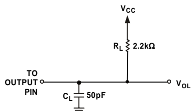
Figure 2. Load Circuit for \overline{BUSY} Timing Diagram
