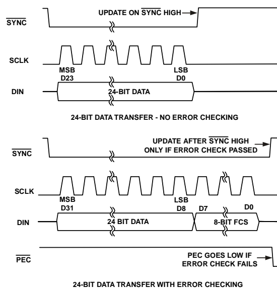
Figure 10. SPI Write With and Without Error Checking
