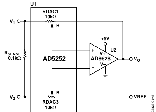
Figure 45. Current-Sensing Amplifier
