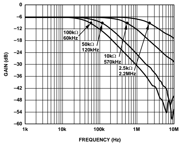
Figure 22. -3 \text{ dB} Bandwidth @ Code = 0x80
