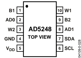
Figure 4. AD5248 Pin Configuration
