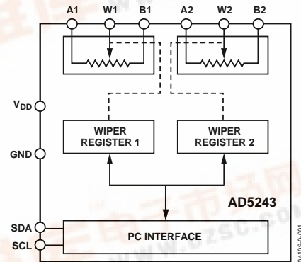
Figure 1. AD5243
