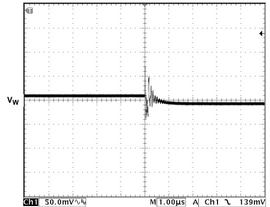
Figure 27. Midscale Glitch, Code 0x80 to 0x7F
