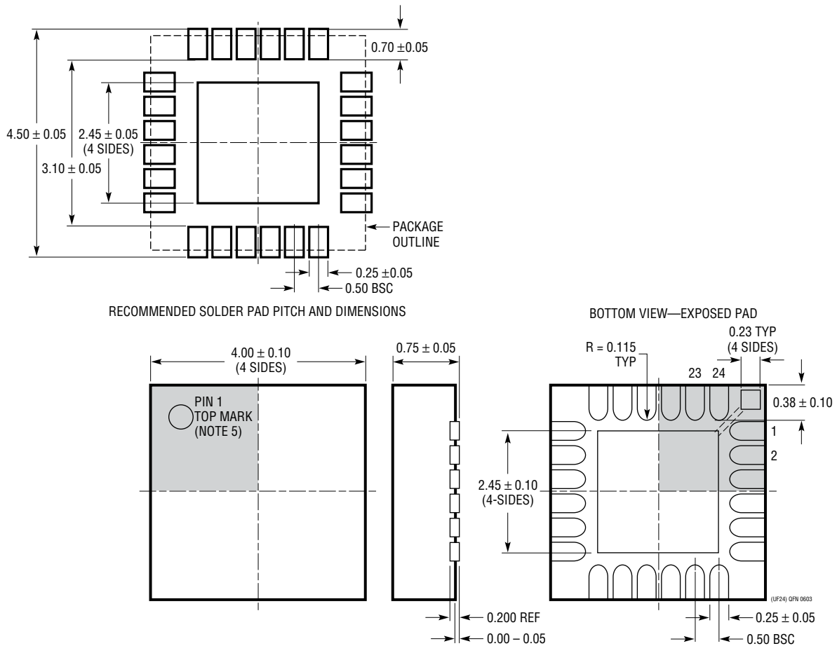
UF Package 24-Lead Plastic QFN (4mm × 4mm) (Reference LTC DWG # 05-08-1697)
