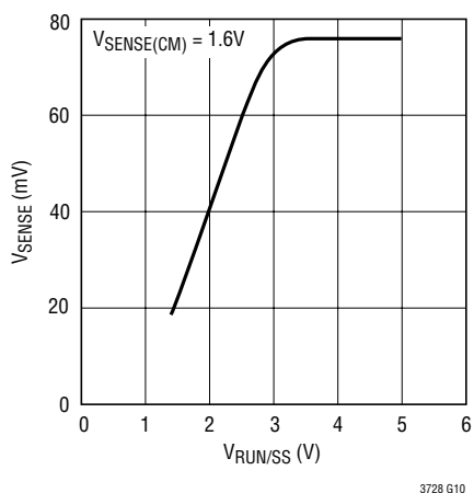
Maximum Current Sense Threshold vs V RUN/SS (Soft-Start)
