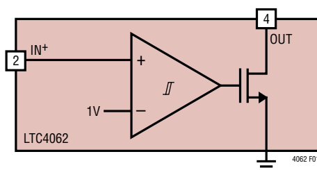
Figure 1. Low Power Comparator Circuit
