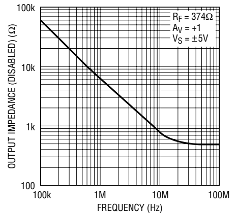
LT1395CS6 Output Impedance (Disabled) vs Frequency
