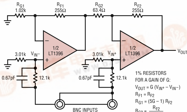
Unity-Gain Video Loop-Through Amplifier
