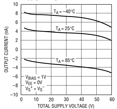
No Load Output Current vs Supply Voltage
