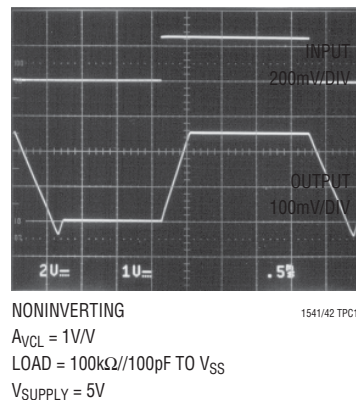
Op Amp Small-Signal Transient Response
