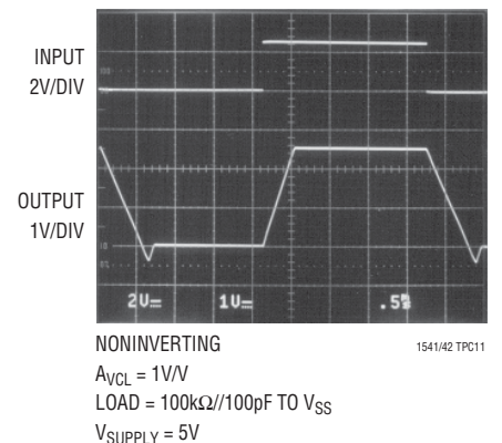
Op Amp Large-Signal Transient Response
