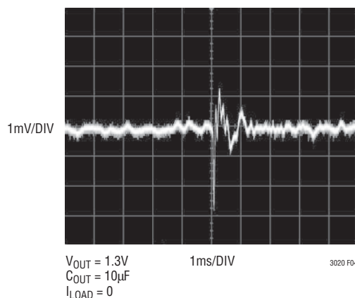
Figure 4. Noise Resulting from Tapping a Ceramic Capacitor
