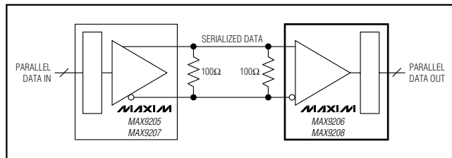
Figure 10. Double-Termination Point-to-Point
