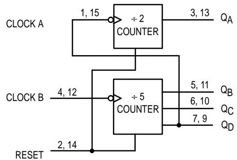
Figure 5. Bi-Quinary Count
