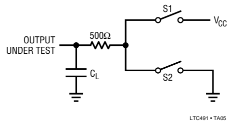
Figure 4. Driver Timing Test Load
