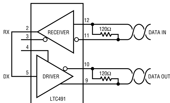
Figure 10. Line Repeater
