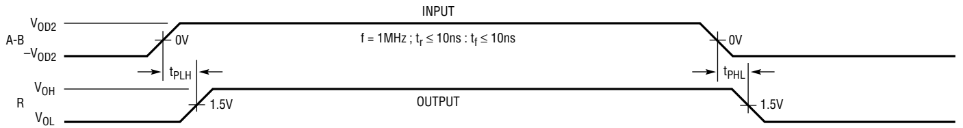
Figure 7. Receiver Propagation Delays
