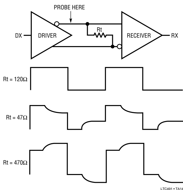
Figure 13. Termination Effects
