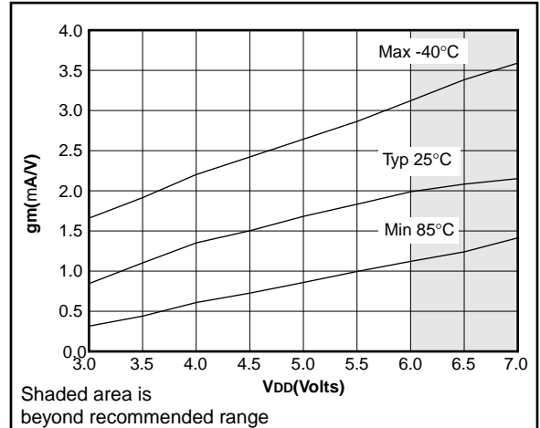
FIGURE 21-20: TRANSCONDUCTANCE(g m ) OF LP OSCILLATOR vs. V DD
