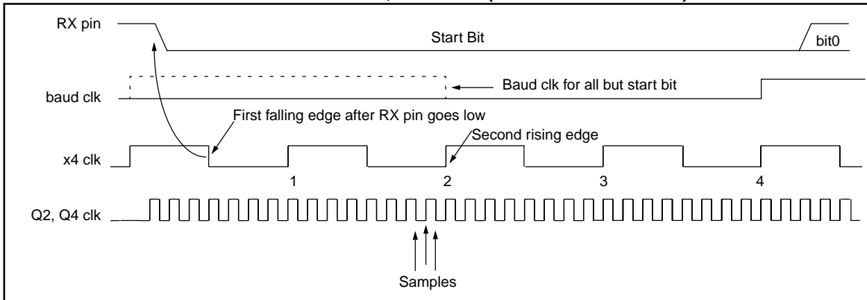
FIGURE 12-5: RX PIN SAMPLING SCHEME, BRGH = 1 (PIC16C73/73A/74/74A)
