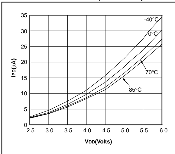
FIGURE 21-4: MAXIMUM IPD vs. VDD (WDT ENABLED, RC MODE)
