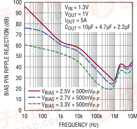
BIAS Pin Ripple Rejection
