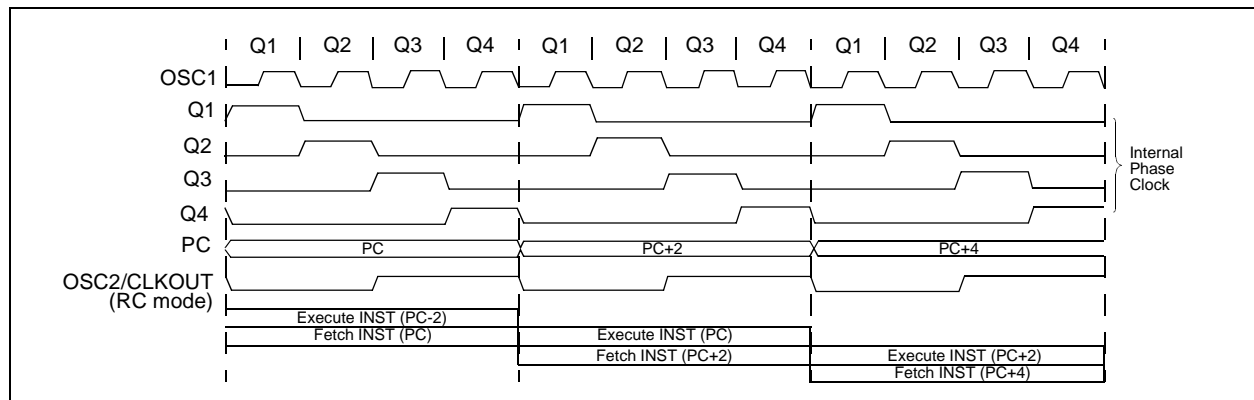
FIGURE 4-4: CLOCK/INSTRUCTION CYCLE
