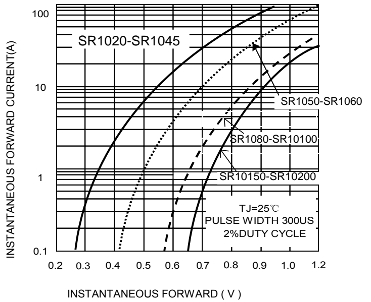
FIG.2-TYPICAL FORWARD CHARACTERISTICS
