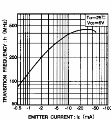
Fig.10 Gain bandwidth product vs. emitter current
