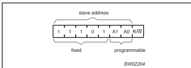
Figure 5. PCA9539 address
