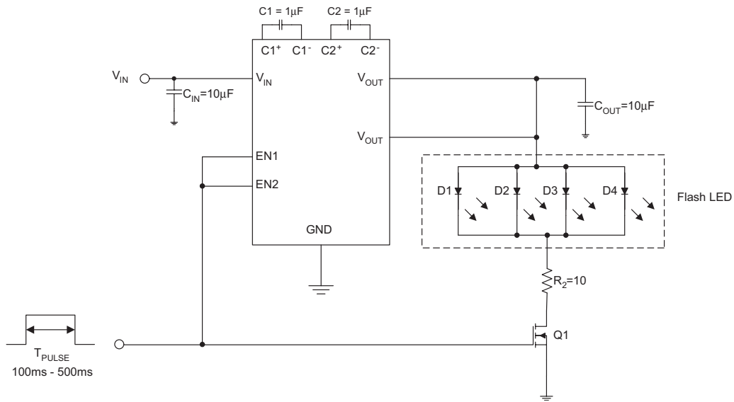
Figure 1: Flash Application.
